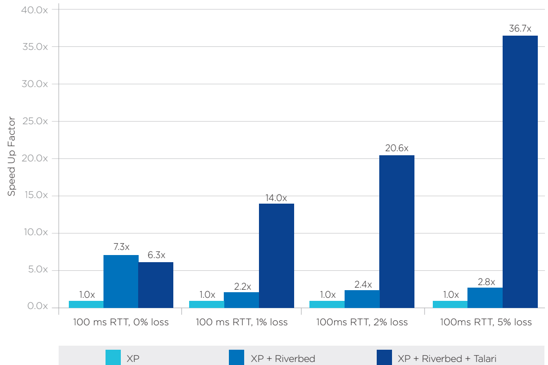
Figure 13 - Windows XP file speed-up factor relative to Windows XP alone for a 40 Mbyte compressible file on a single 20 Mbps link for different loss rates with 100 ms RTT when using Riverbed (cold) and Talari appliances
