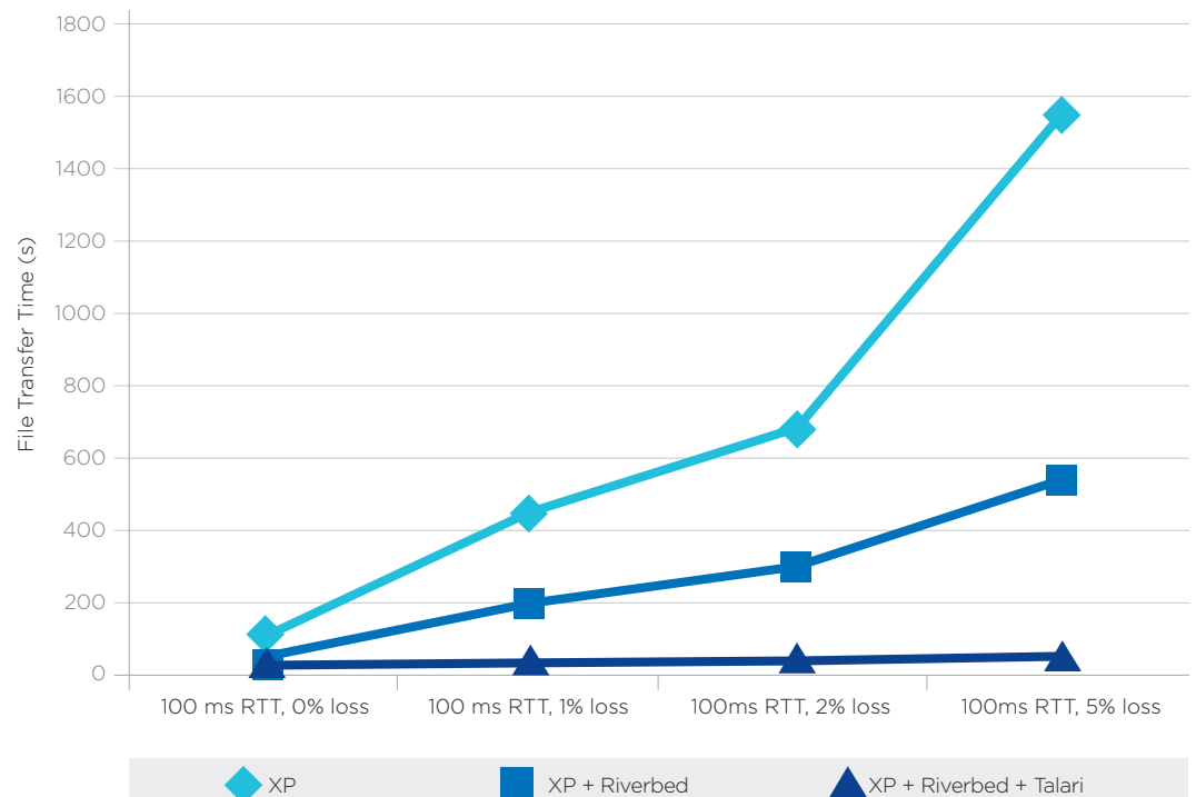
Figure 12 - Windows XP file transfer time for a 40 Mbyte compressible file on a single 20 Mbps link for different loss rates with 100 ms RTT when using Riverbed (cold) and Talari appliances
