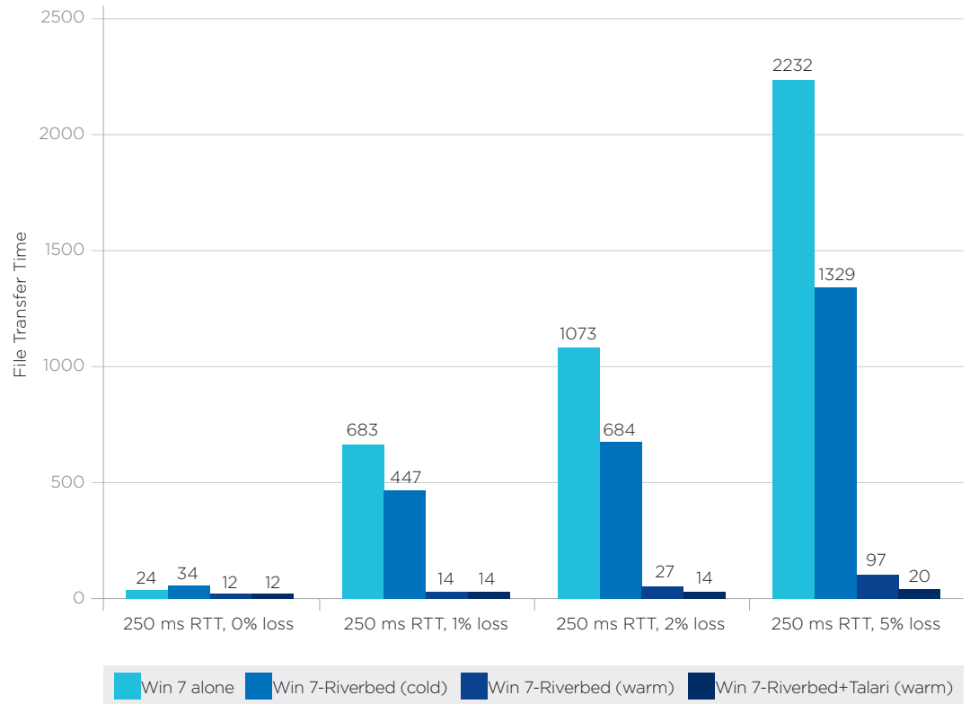
Figure 4 - Windows 7 file transfer times for a compressible 40 Mbyte file on a 20 Mbps link for different loss rates with 250 ms RTT when using Riverbed and Talari appliances
