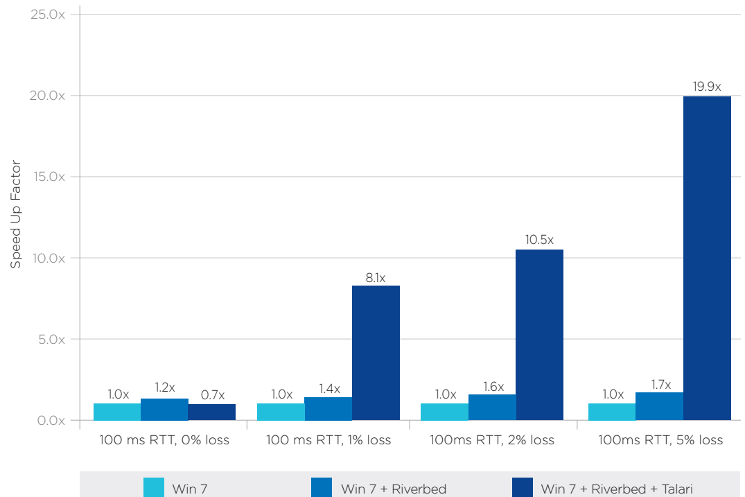
Figure 15 - Windows 7 file speed-up factor relative to Windows 7 alone for a 40 Mbyte compressible file on a single 20 Mbps link for different loss rates with 100 ms RTT when using Riverbed (cold) and Talari appliances
